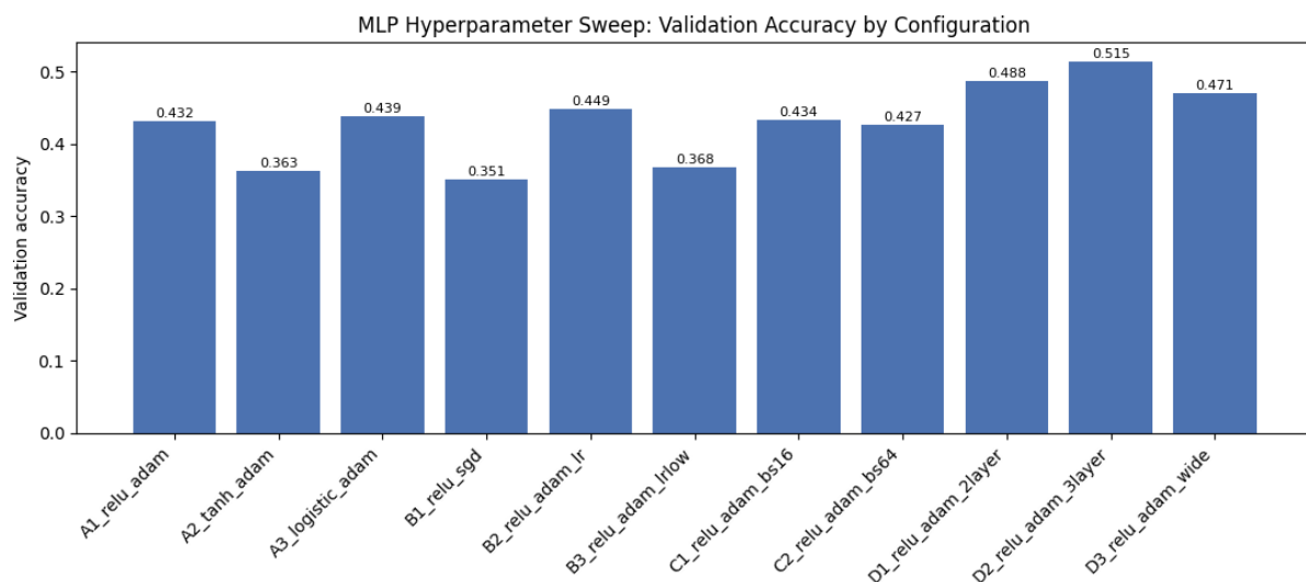
Figure 2: Validation accuracy across the 11-configuration hyperparameter sweep.
